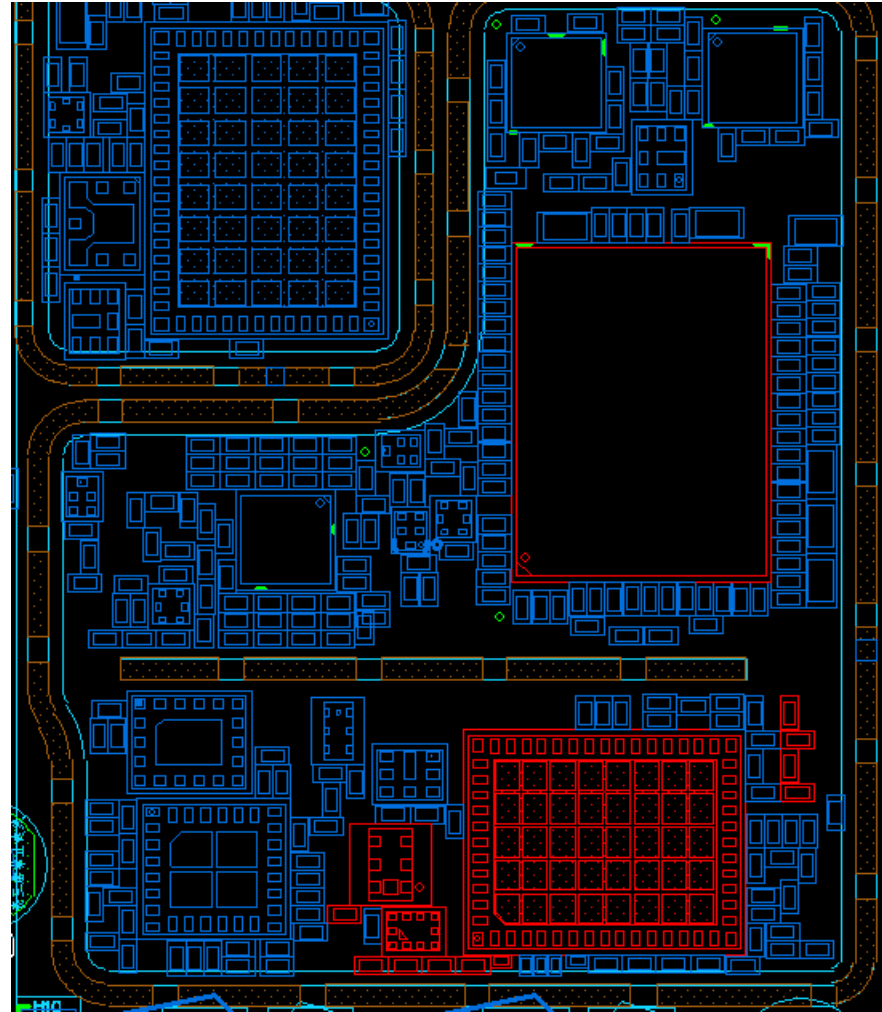
LB + B1/B3/B7 DiPX U4503
