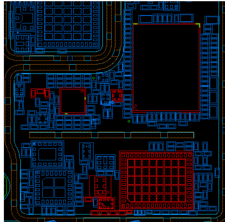
LB + B1B3B7 DiPX U4503
