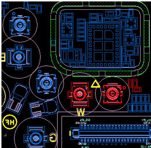
RF Connector LB J4501 J4502
