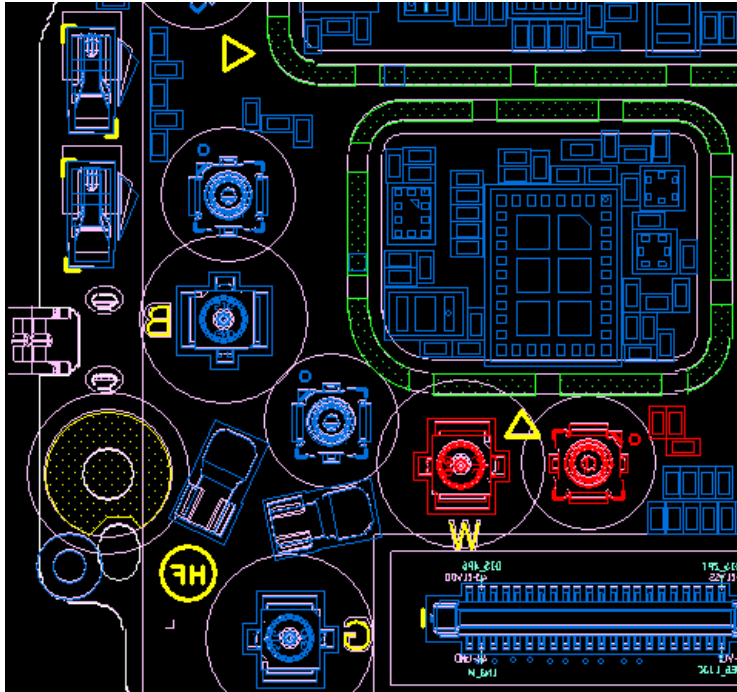
RF Connector LB J4501 J4502
